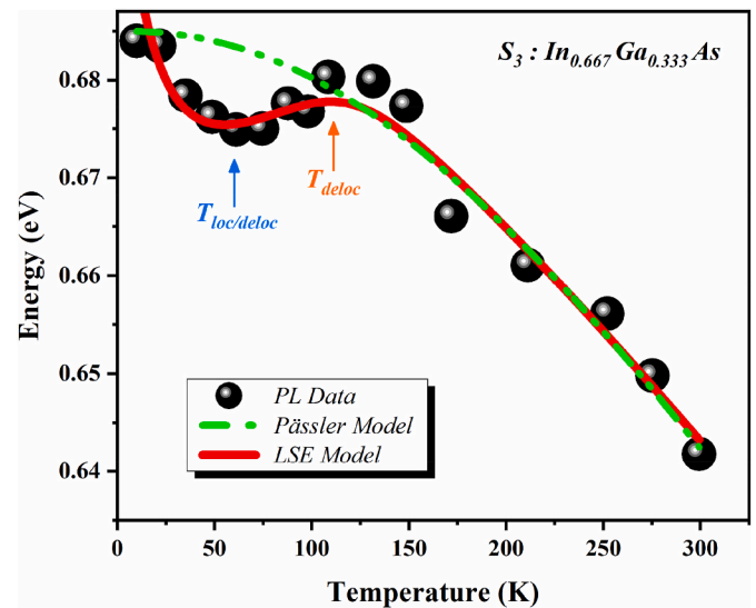
Fig. 5. Temperature dependence of steady-state photoluminescence energy for S_3 : Comparison between semi-empirical Pässler model and LSE model.
