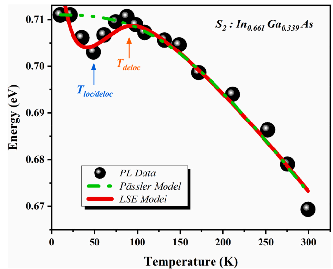
Fig. 4. Temperature dependence of steady-state photoluminescence energy for S_2 : Comparison between semi-empirical Pässler model and LSE model.
