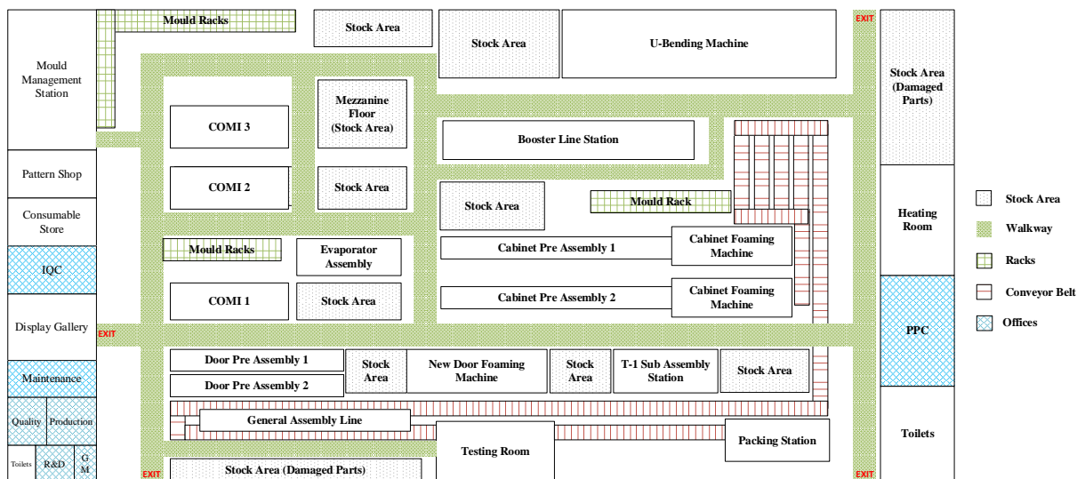
Figure 8: Improved Layout
