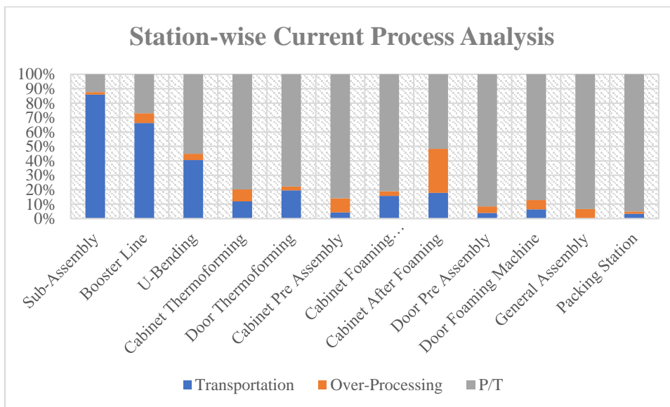
Figure 4: Station-wise Current Process Analysis
