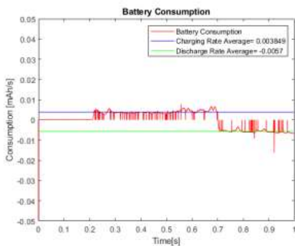
Fig. 14- Battery Consumption Rate Driven by Random Vibration
