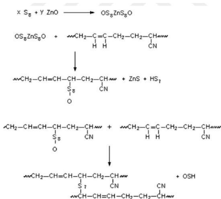
Figure 5: Structure of S vulcanization by NBR (Passador et al., 2009).
