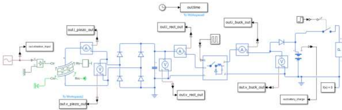
Fig.2- Piezoelectric Principle Based Energy Harvesting System Simulink Model
