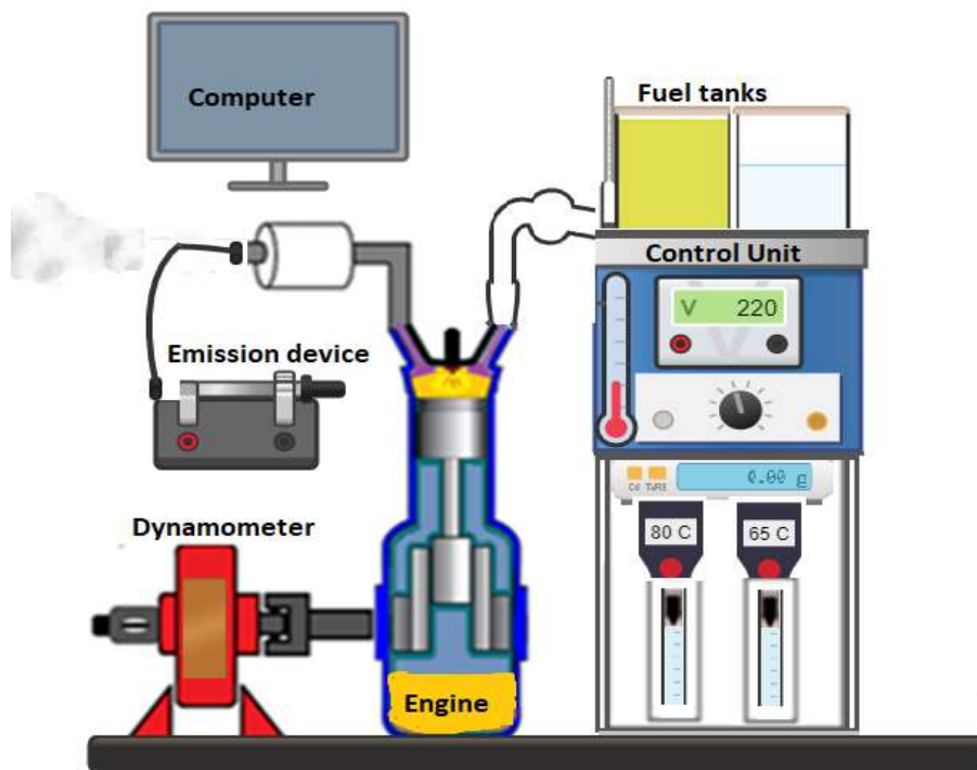
Figure 3. Experimental setup.
