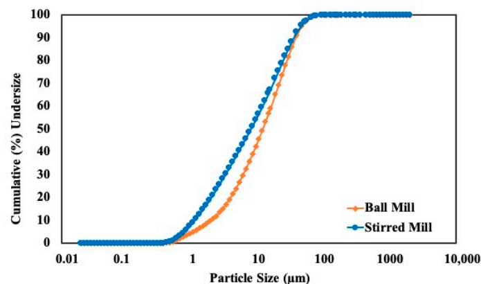
Figure 8. Particle size distributions of products for calcite grinding by stirred mill and ball mill.
