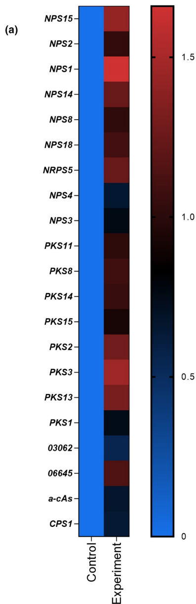
FIGURE 5 Specific transcripts related to characteristic pathways obtained from enrichment analysis. [Colour figure can be viewed at wileyonlinelibrary.com ]
