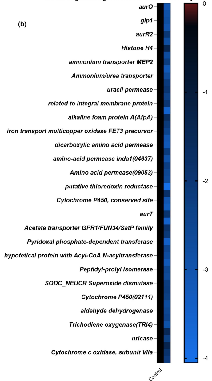
FIGURE 5 Specific transcripts related to characteristic pathways obtained from enrichment analysis. [Colour figure can be viewed at wileyonlinelibrary.com ]
