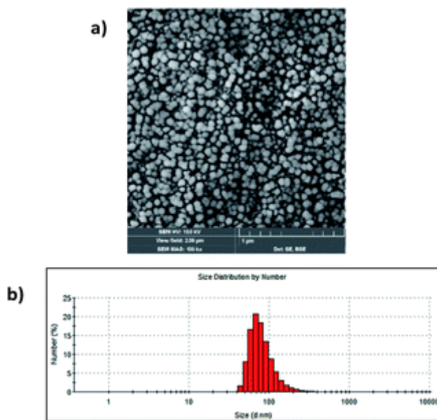
Fig. 2 (a) SEM image of VP-Afrrt-CuS nanoparticles stained with 2% uranyl acetate. (b) The size distribution of VP-Afrrt-CuS nanoparticles.
