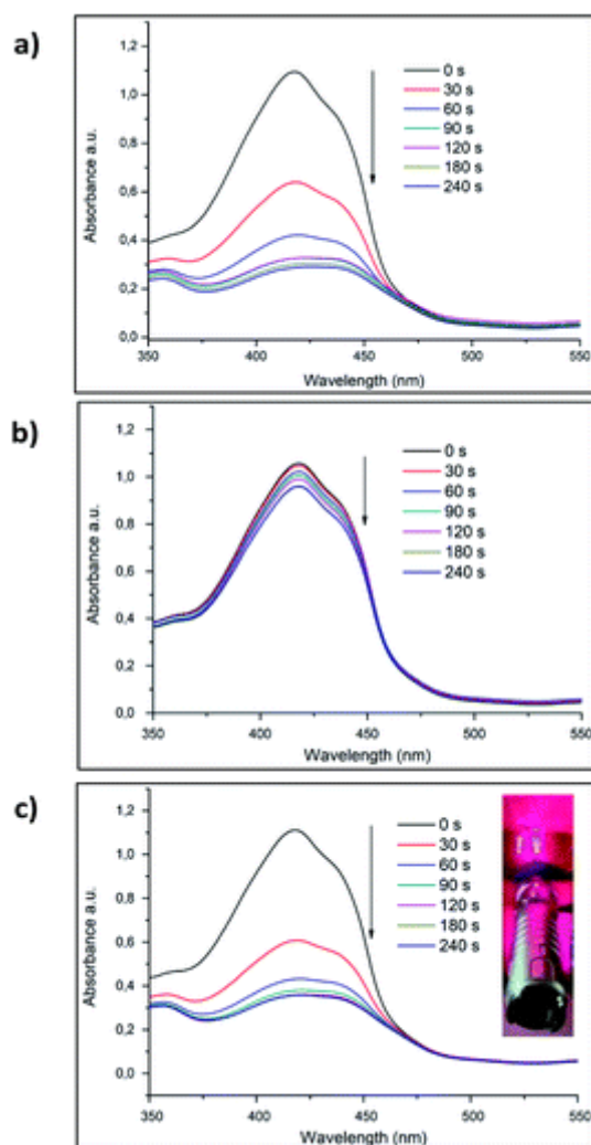
Fig. 3 (a) Decrease in the absorbance of DPBF in the presence of 22.5 \text{ mg mL}^{-1} VP-Afrr-CuS nanoparticles (total volume 250 \mu\text{L} ) at 416 \text{ nm} in DMSO after irradiated with 690 \text{ nm} LED. (b) Decrease in the absorbance of DPBF in the presence of 22.5 \text{ mg mL}^{-1} VP-Afrr-CuS nanoparticles (total volume 250 \mu\text{L} ) at 416 \text{ nm} in DMSO after irradiated with 808 \text{ nm} ( 1.5 \text{ W cm}^{-2} ) laser. (c) Decrease in the absorbance of DPBF in the presence of 22.5 \text{ mg mL}^{-1} VP-Afrr-CuS nanoparticles (total volume 250 \mu\text{L} ) at 416 \text{ nm} in DMSO after irradiated with 808 \text{ nm} ( 1.5 \text{ W cm}^{-2} ) laser and 690 \text{ nm} LED, simultaneously. Inset: irradiation of VP-Afrr-CuS nanoparticles with 808 \text{ nm} ( 1.5 \text{ W cm}^{-2} ) laser and 690 \text{ nm} LED, simultaneously.
