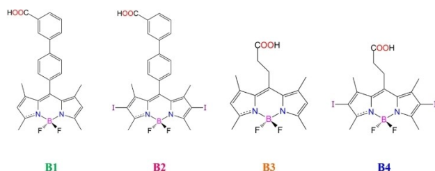
Scheme 1. Schematic illustration of the BODIPY sensitizers.
